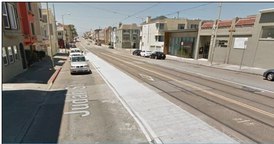
Judah Street boarding island (with mountable curb)
