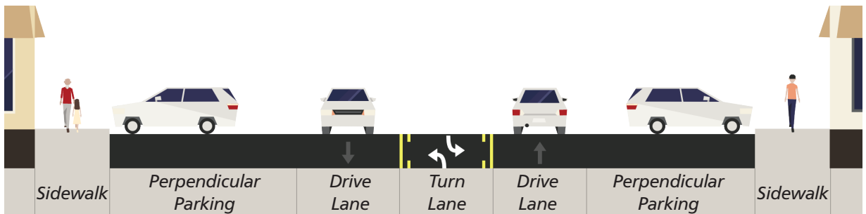
Typical Proposed Street Configuration (looking west)
