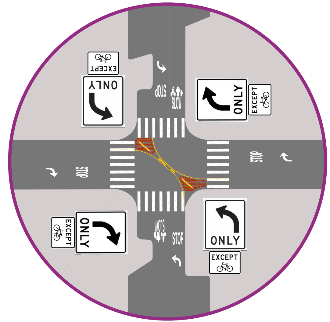
Option 2: Diagonal Diverter
