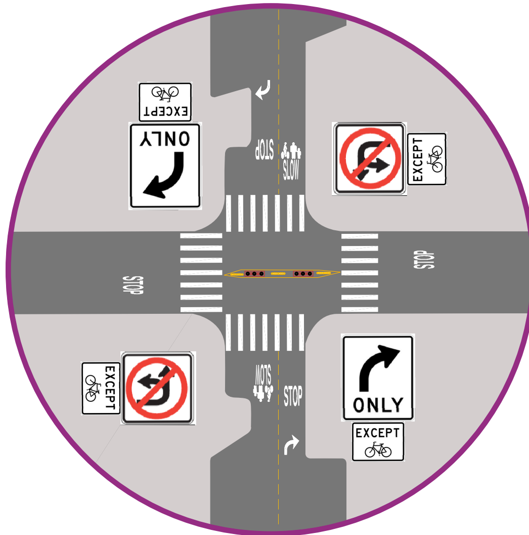
Option 1: Median Diverter
